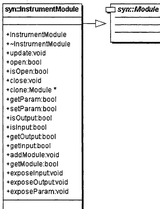
Figure 30. UML diagram for the Instrument type.
