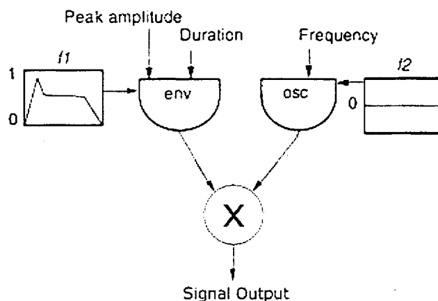
Figure 13. Example of a multiplier used to control amplitude.
